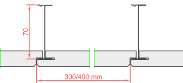
Length panels 2500 mm
